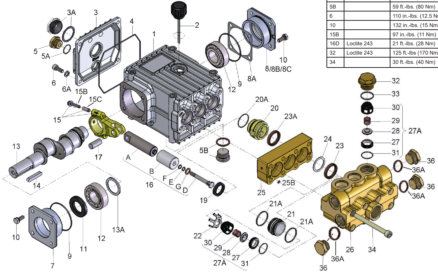
Exploded View - P470A/P490A
